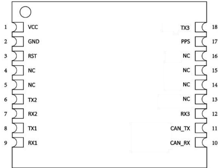
IMU614E- AG Pin Layout (Top View)
